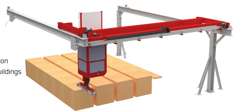
Configuration C Cantilever crane on fixed framework
